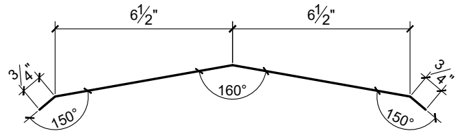
CROSS SECTION
