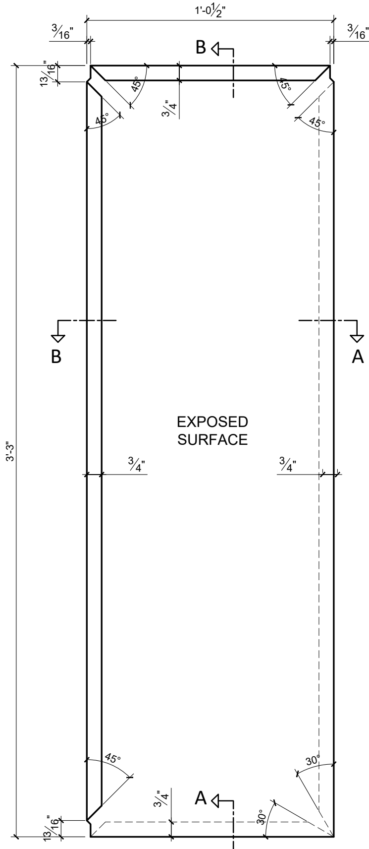
PLAN VIEW
